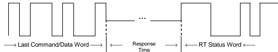
Figure 5-6 RT Response Time Definition
