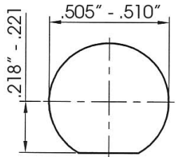
RECOMMENDED MOUNTING HOLE (inches)
